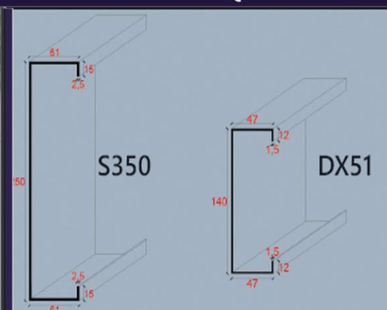
LIGHT STEEL PROFILE SECTION
