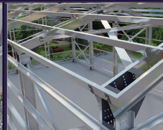
ROOF-CORNER PURLIN CONNECTION
