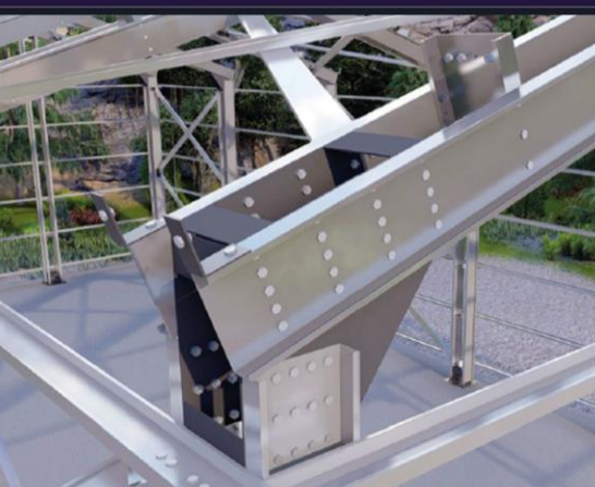
ROOF- CORNER PURLIN EQUIPMENT
