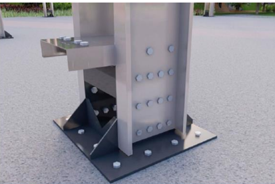
GROUND CONNECTION DETAIL
